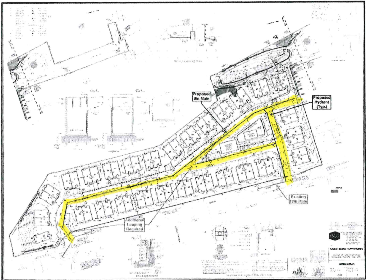
Figure 5 Site Development Plan (Provided By Developer)
